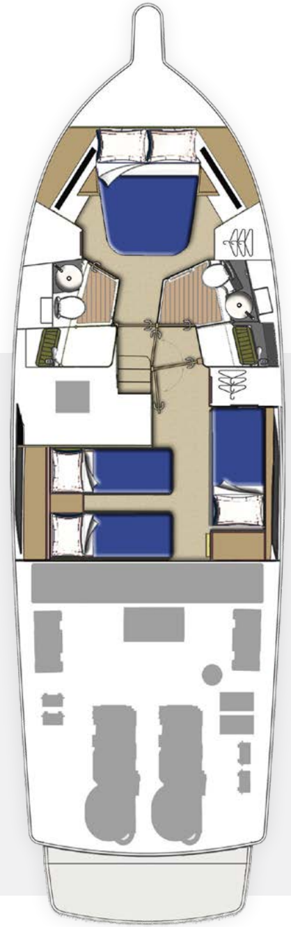
ACCOMMODATION DECK
